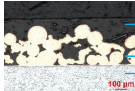
Photomicrograph of the 3-layer material (steel back + sliding layer of porous bronze + compound of thermoplastic (PEEK), PTFE, C-fibres and graphite)
